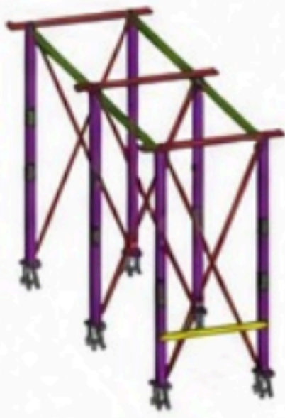
BRACED FRAME
